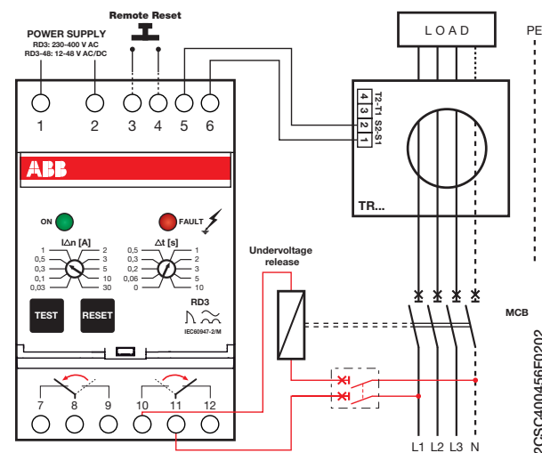
Connection to undervoltage release
