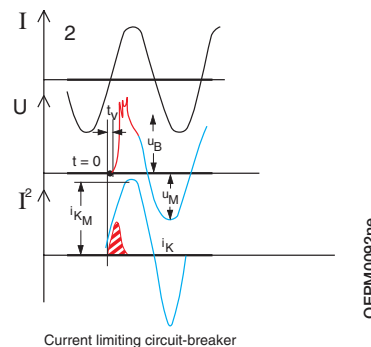
Current limiting circuit-breaker
