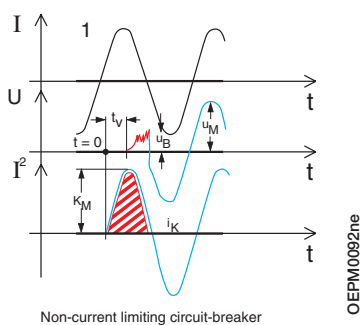
Non-current limiting circuit-breaker
