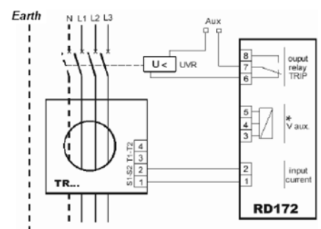
Example of wiring diagram: shunt trip connection and undervoltage release (fail safe OFF)
