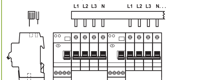
PS 4/36/16 H-DDA 204 T DS 204 (≤ 40 A) + S2C-S/H6R + DS 204 (≤ 40 A) + S2C-S/H6R + DDA 204 (≤ 40 A) + S 204 + S2C-S/H6R + DDA 204 (≤ 40 A) + S 204 + S2C-S/H6R
