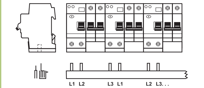
PS 3/26/16H-DDA 202 DS 202 + S2C-S/H6R + DS 202 + S2C-S/H6R + DDA 202 + S 202 + S2C-S/H6R + DDA 202 + S 202 + S2C-S/H6R ...
